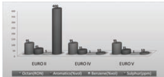
Gasoline chart comparison with standard EURO II and EURO IV and EURO V
