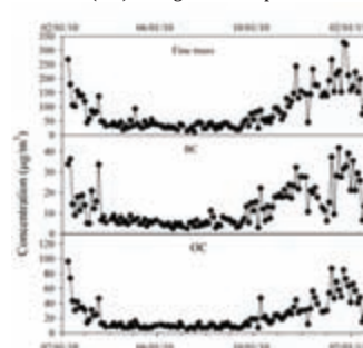
Variation of PM fraction (FPM), black carbon (BC) and organic carbon (OC) during 2010-2011 period
