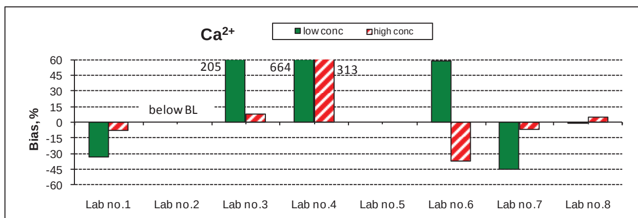
Fig.10 Distribution of Ca 2+ data normalized by prepared value (off-scale values are indicated, %)
