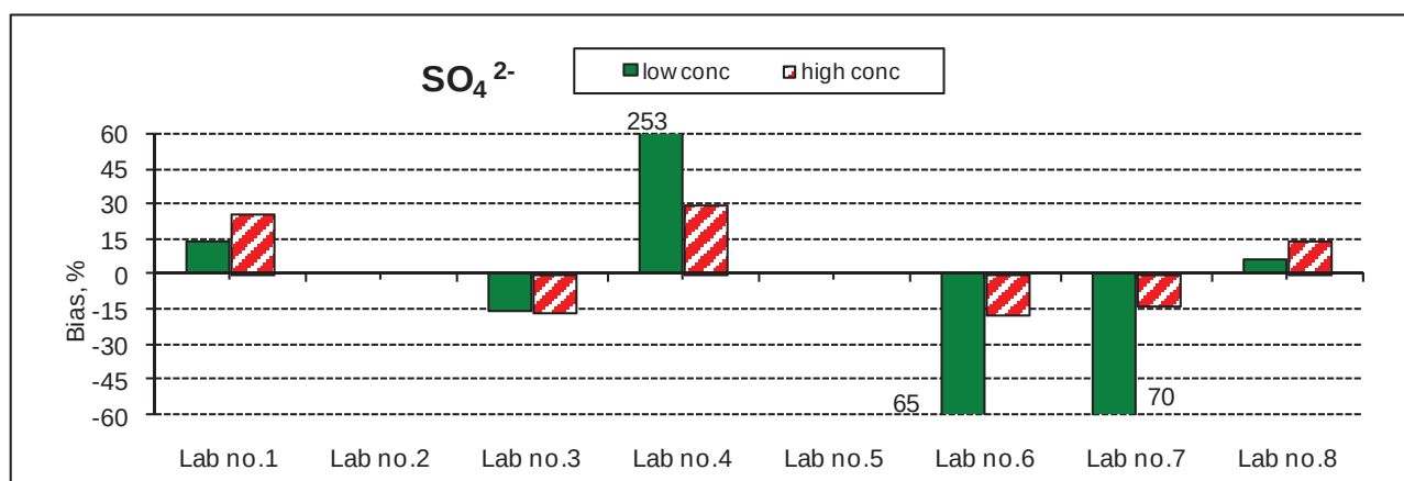
Fig.5 Distribution of \text{SO}_4^{2-} data normalized by prepared value (off-scale values are indicated, %)
