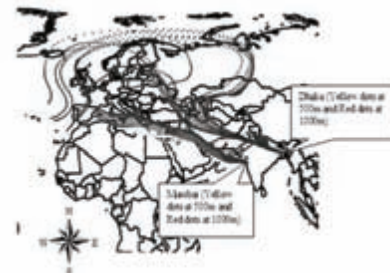
Air parcel back trajectories showing long range transport of soil dust in Bangladesh and India in February 2003
