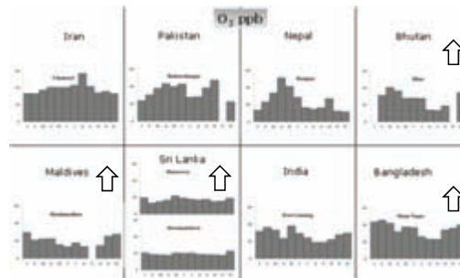
Ozone concentrations with IVL Passive Samplers at Malé Declaration regional sites, monthly means 2006-2012
