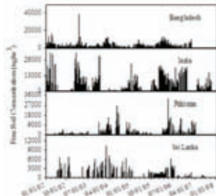
Time series plots of fine soil concentrations in Bangladesh, India, Pakistan and Sri Lanka
