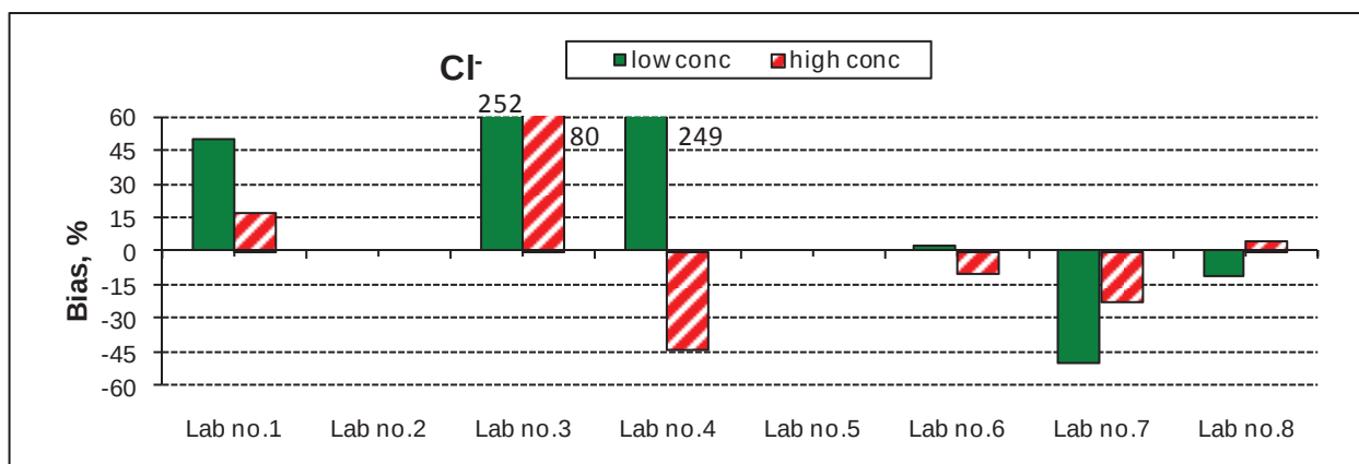
Fig.7 Distribution of Cl - data normalized by prepared value (off-scale values are indicated, %)
