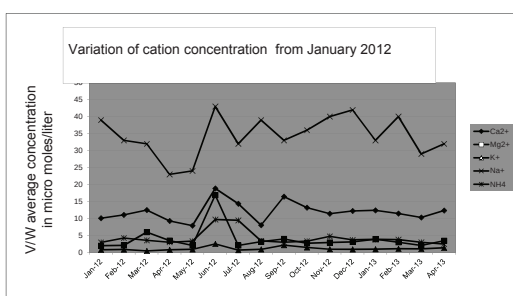
Wet deposition monitoring data
