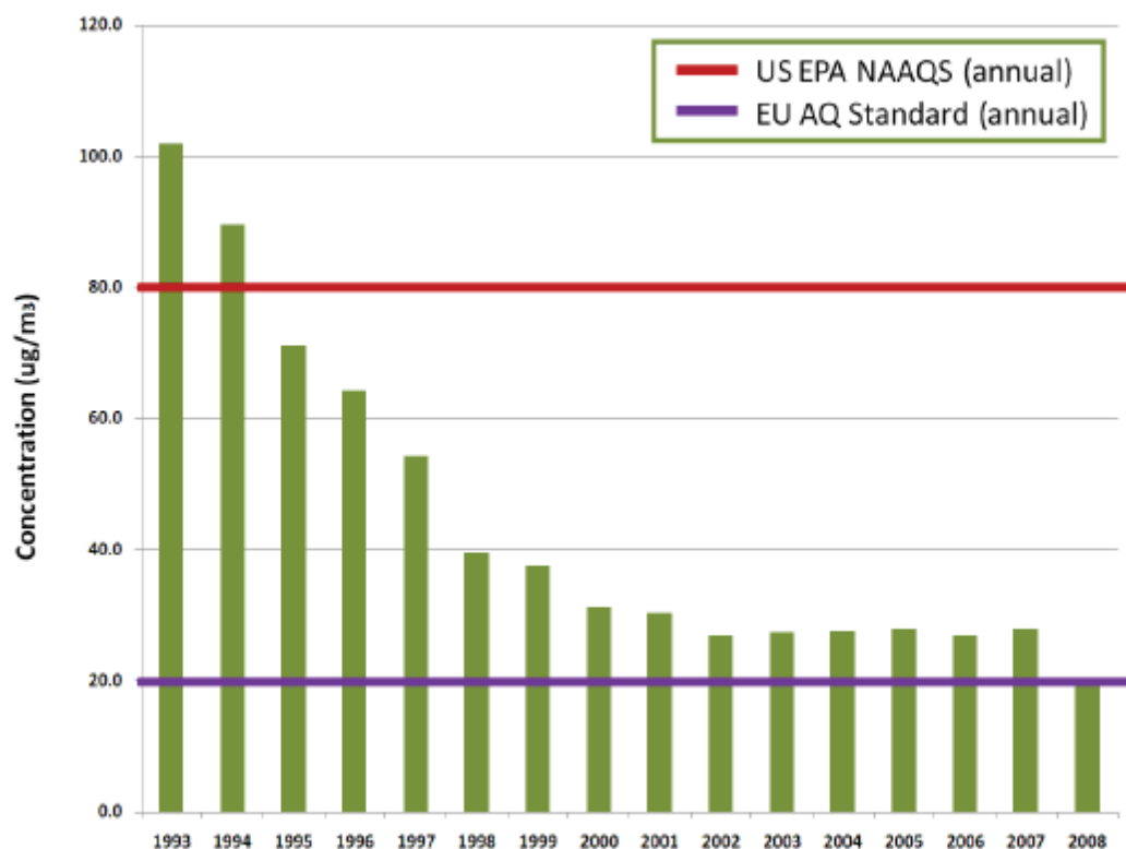
Average of Annual Average Annual Ambient AQ in Selected Asian Cities (1993-2008), CAI-ASIA 2010
