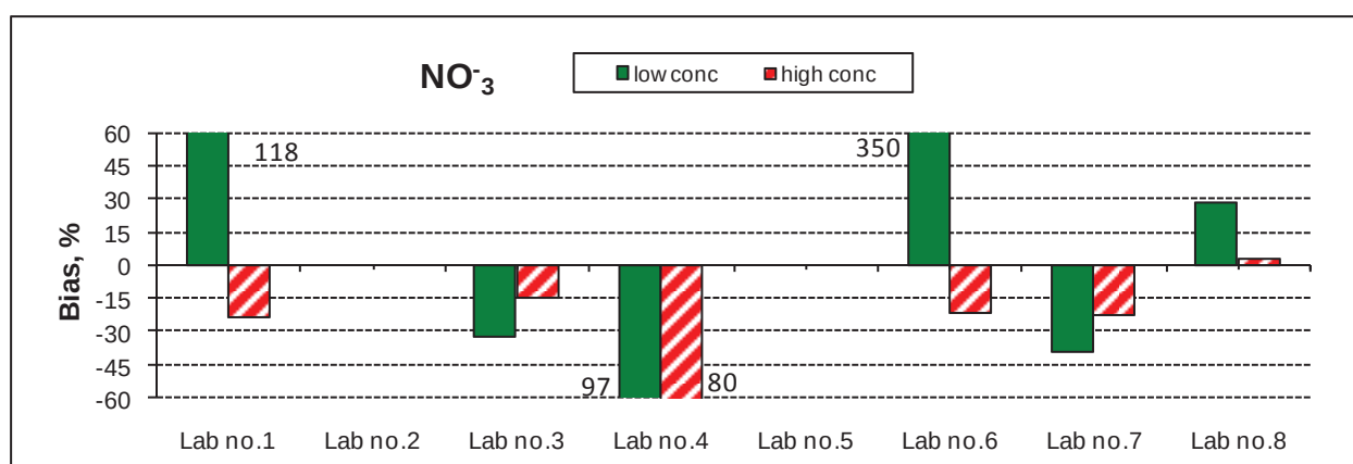
Fig.6 Distribution of \text{NO}_3^- data normalized by prepared value (off-scale values are indicated)
