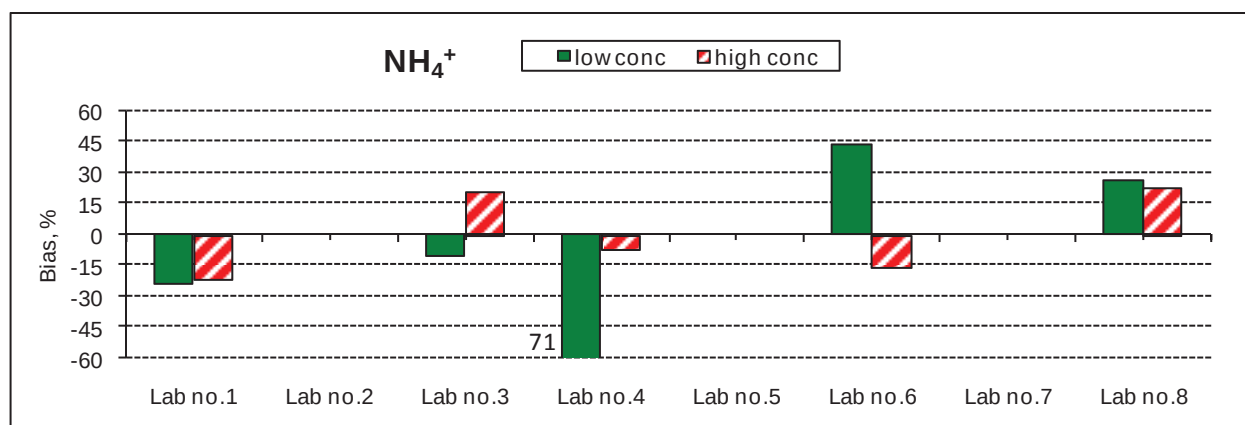
Fig.12 Distribution of \text{NH}_4^+ data normalized by prepared value (off-scale values are indicated, %)
