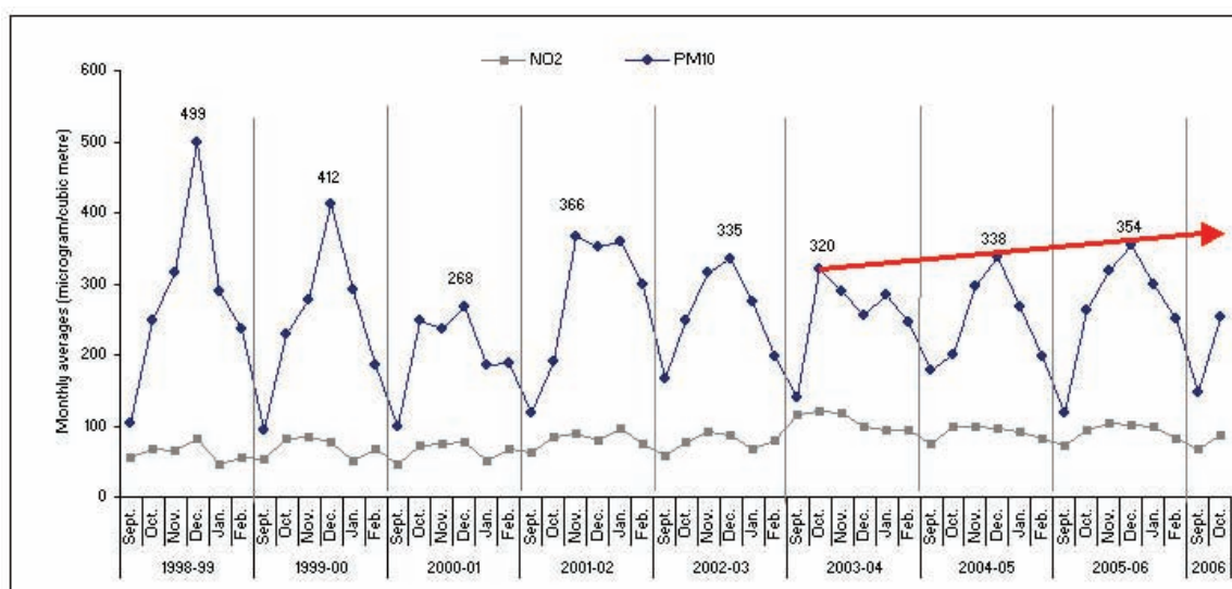
Figure 2.8: Trend of NOx and PM in Delhi
