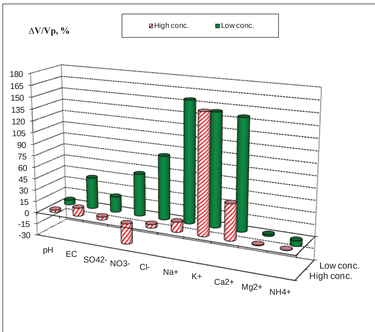
Fig.13 Relative deviation between average submitted data and prepared value [\Delta V = \text{Average } (V_a) - \text{Prepared } (V_p)]
