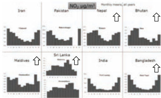
Nitrogen dioxide concentrations with IVL Passive Samplers at Malé Declaration regional sites, monthly means 2003-2012
