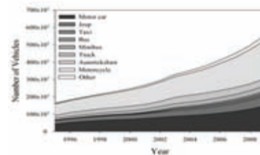
Year-by-year registration of vehicles in Dhaka City (Source: Bangladesh Road Transport Authority, 2010)
