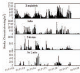
Time series plots of fine Smoke contribution
