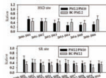
Ratios of PM 2.5 /PM 10 and BC/PM 2.5 over the collection periods from April 2000 to March 2006 and April 2000 to March 2010 at HS and SR sites
