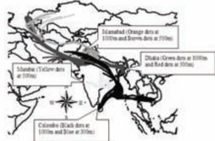
Air parcel back trajectories showing the likely sources areas for smoke
