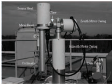
Figure 1: Cornet sun photometer with sensor head and data cable attached
