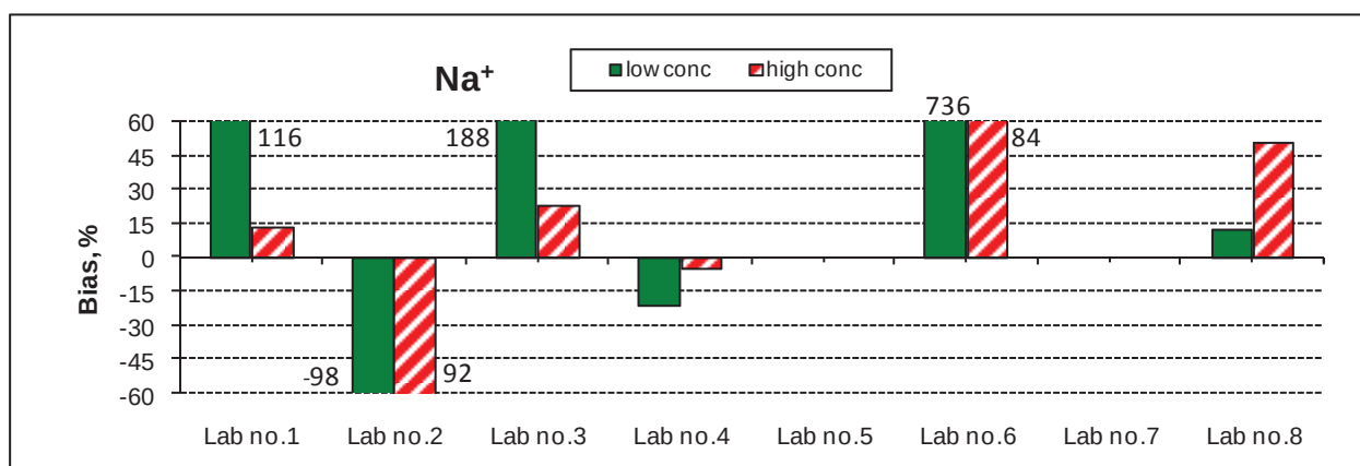
Fig.8 Distribution of Na + data normalized by prepared value (off-scale values are indicated)
