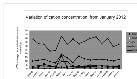
Wet deposition monitoring data
