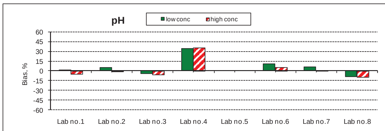
Fig.3 Distribution of pH data normalized by prepared value
