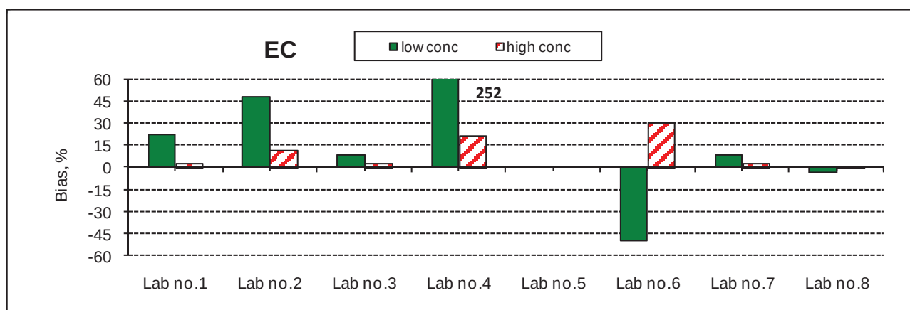
Fig.4 Distribution of EC data normalized by prepared value (off-scale values are indicated, %)
